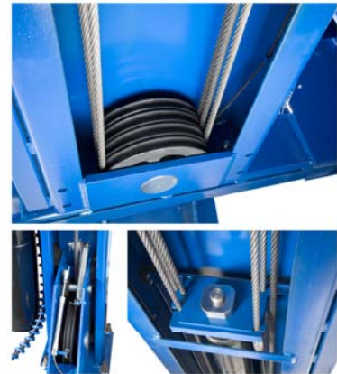
HD-Series Super-Duty Four Post Details
