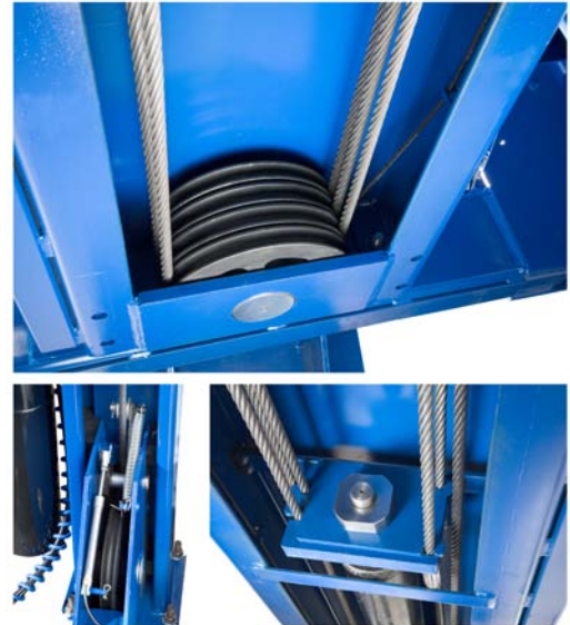
HD-Series Super-Duty Four Post Details
